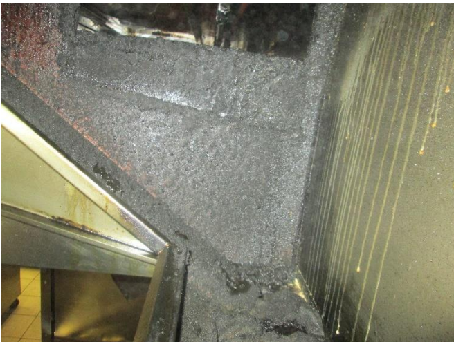
Ductwork riser from main canopy
